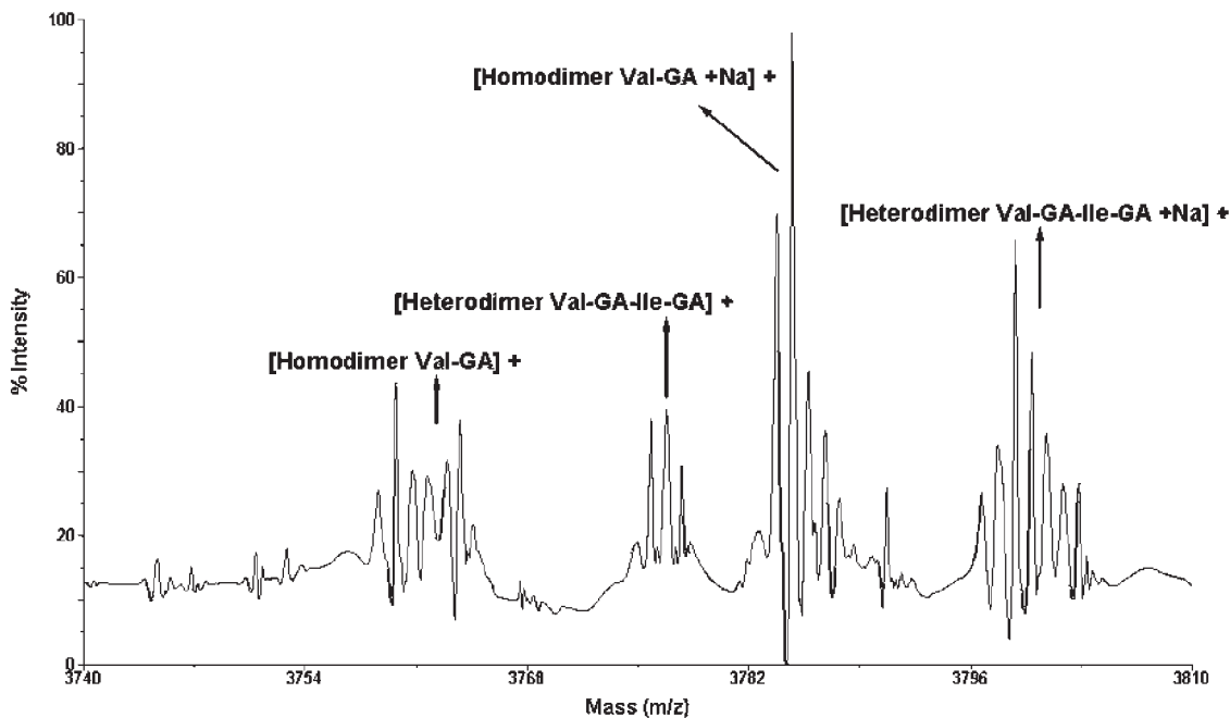
FIGURE 5 MALDI-TOF mass spectrum of gramicidin D from methanol solution in the m/z 3740–3810 range showing homo- and heterodimers.
