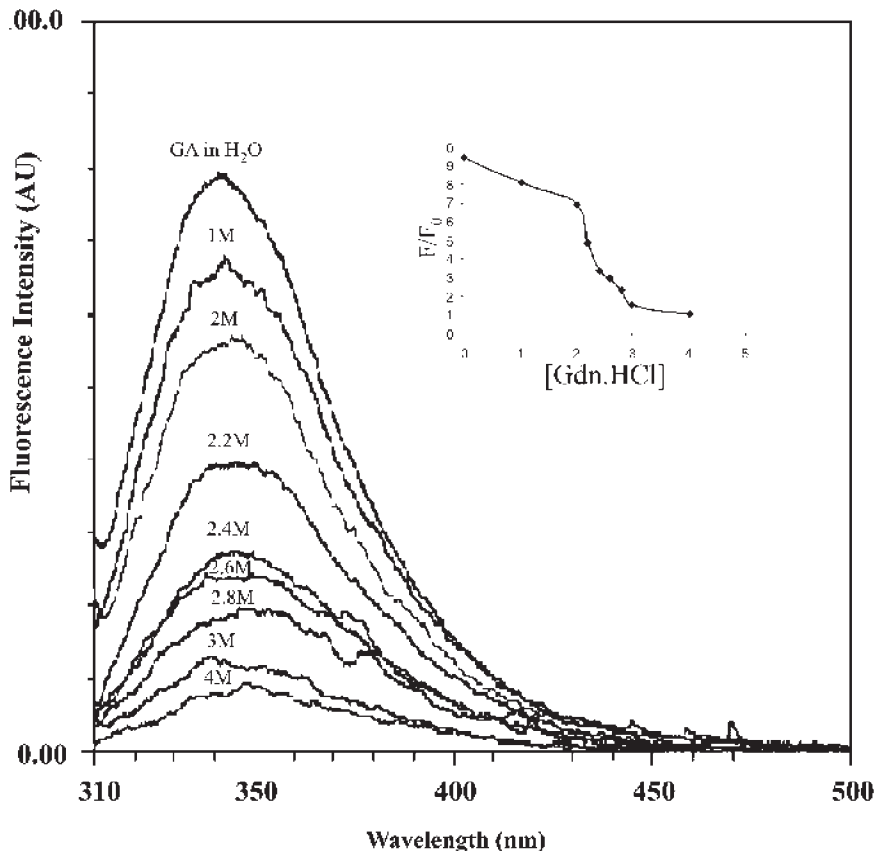
FIGURE 3 Emission spectra and (inset) changes in fluorescence intensity of gramicidin D (2 \mu M) as a function of guanidinium hydrochloride (Gdn · HCl) concentration.
